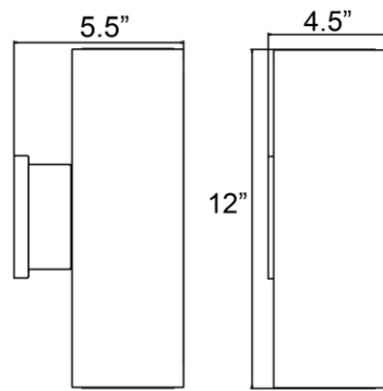
LINE DRAWING
